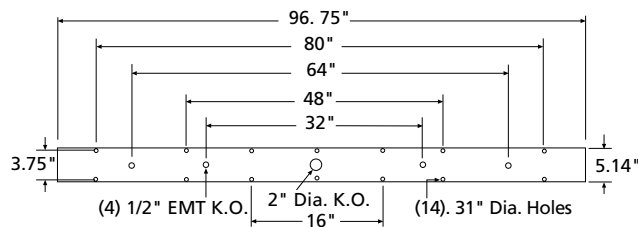
MOUNTING HOLES
