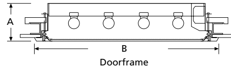
CROSS SECTION
