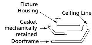
GASKET PROFILE
