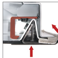
Section View
